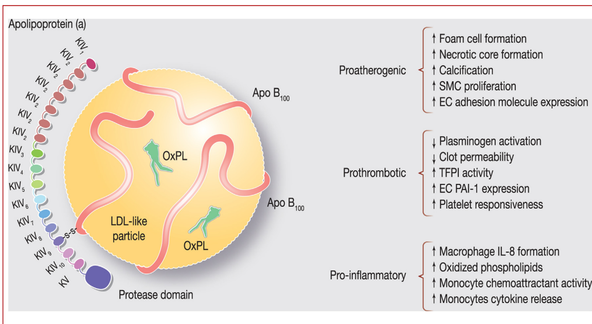
Figure 1. Lipoprotein(a) structure. Apo: apolipoprotein; EC: endothelial cell; IL: interleukin; KIV: kringle IV; KV: kringle V; LDL: low-density lipoprotein; OxPL: oxidised phospholipids; PAI: plasminogen activator inhibitor; SMC: smooth muscle cell; TFPI: tissue factor pathway inhibitor.
